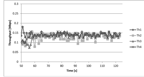
Figure 19: proposal - short-term throughput
