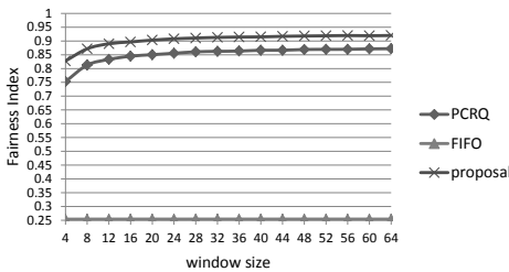
Figure 9: Fairness Index
