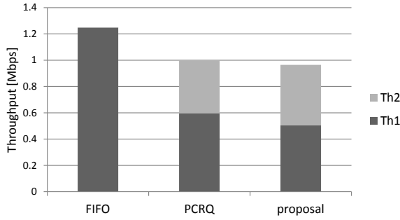
Figure 7: Throughput scenario 1
