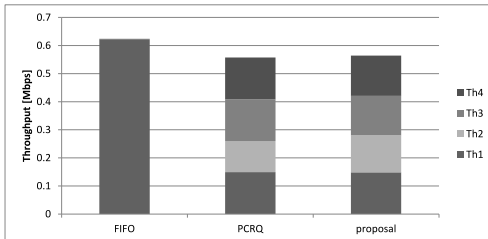
Figure 16: Throughput scenario 3
