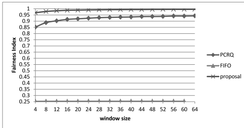
Figure 15: Fairness Index
